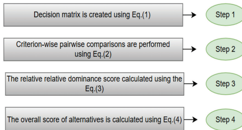
Figure 1. Flowchart of the proposed RPR method
