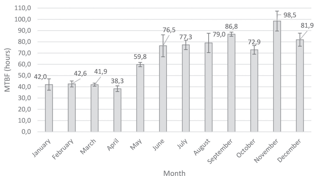
Figure 1. Monthly MTBF (hours) of Wood Chipper 1 with 95% confidence intervals.
