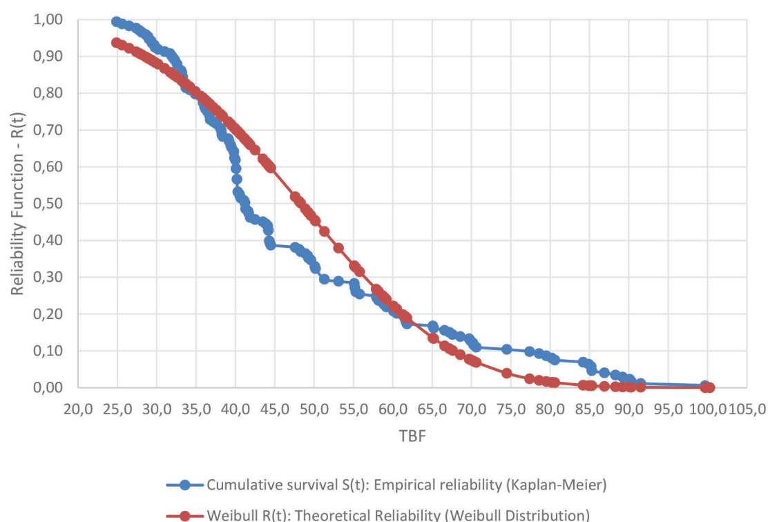
Figure 4. Comparison between the Kaplan-Meier survival curve and the Weibull model for the Wood Chipper 1.
