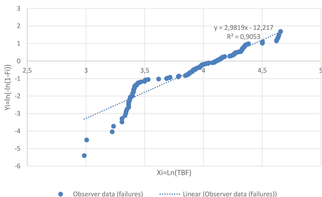
Figure 10. Weibull probability plot for Wood Chipper 2.
