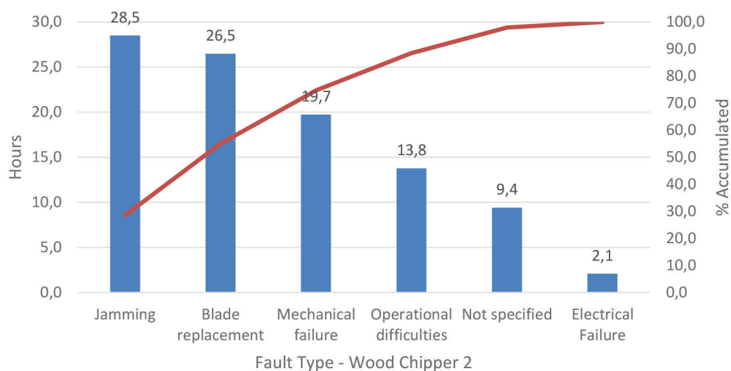
Figure 12. Analysis of various types of Wood Chipper 2 failures using the Pareto Diagram.
