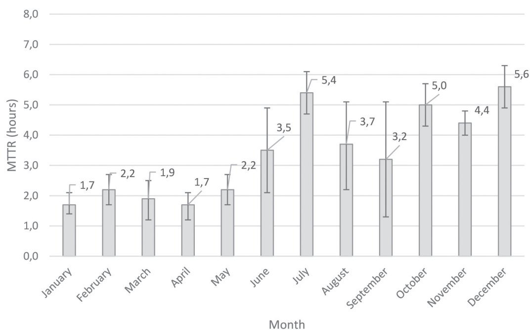
Figure 2. Monthly MTTR (hours) of Wood Chipper 1 with 95% confidence intervals.
