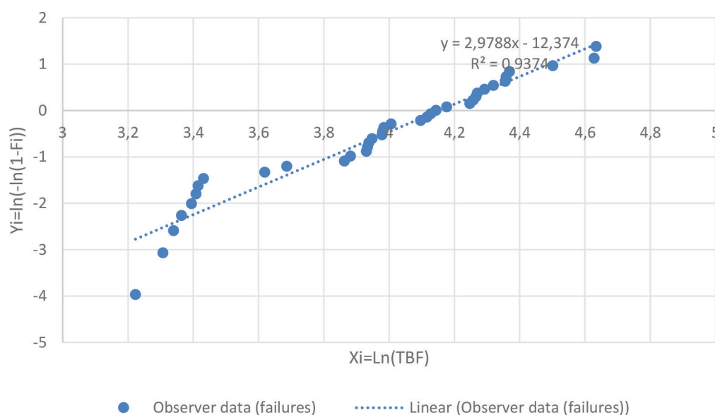
Figure 13. Weibull probability plot fitted exclusively to blade replacement failures in Wood Chipper 2.
