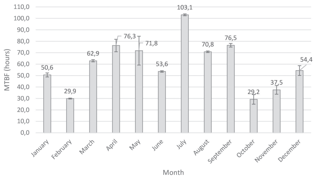
Figure 8. Monthly MTBF (hours) of Wood Chipper 2 with 95% confidence intervals.
