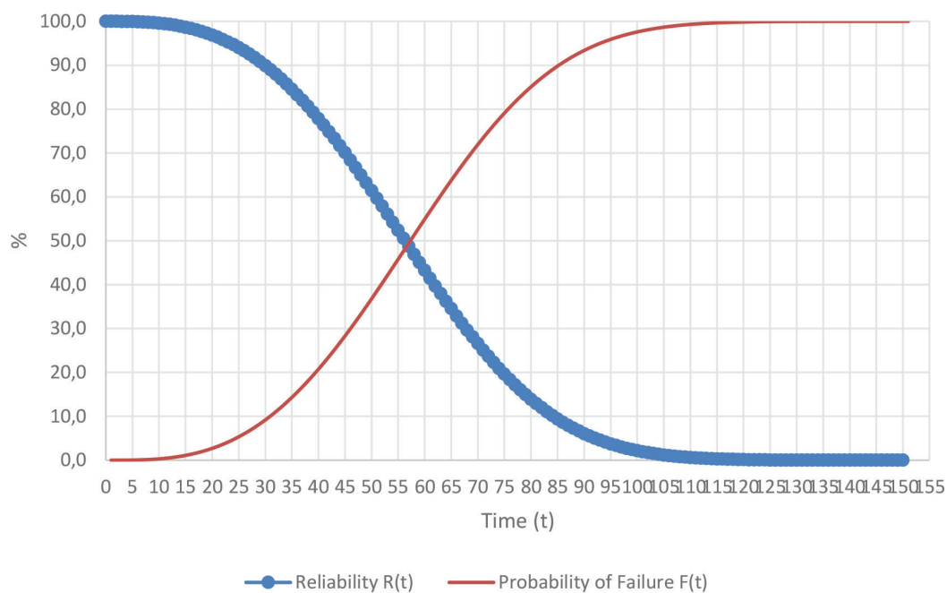
Figure 14. Cumulative failure functions F(t) and reliability R(t) of the Wood Chipper 2.
