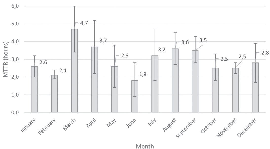
Figure 9. Monthly MTTR (hours) of Wood Chipper 2 with 95% confidence intervals.
