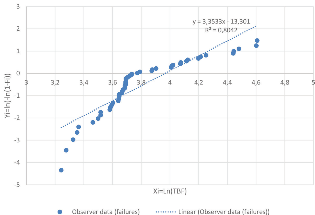
Figure 6. Weibull probability plot fitted exclusively to blade replacement failures in Wood Chipper 1.
