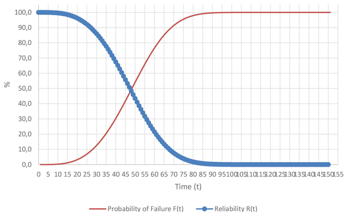
Figure 7. Cumulative failure functions F(t) and reliability R(t) of the Wood Chipper 1.
