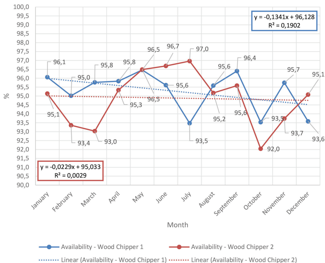
Figure 15. Monthly operational availability of wood chippers 1 and 2 over a 12-month period, with linear trend lines.
