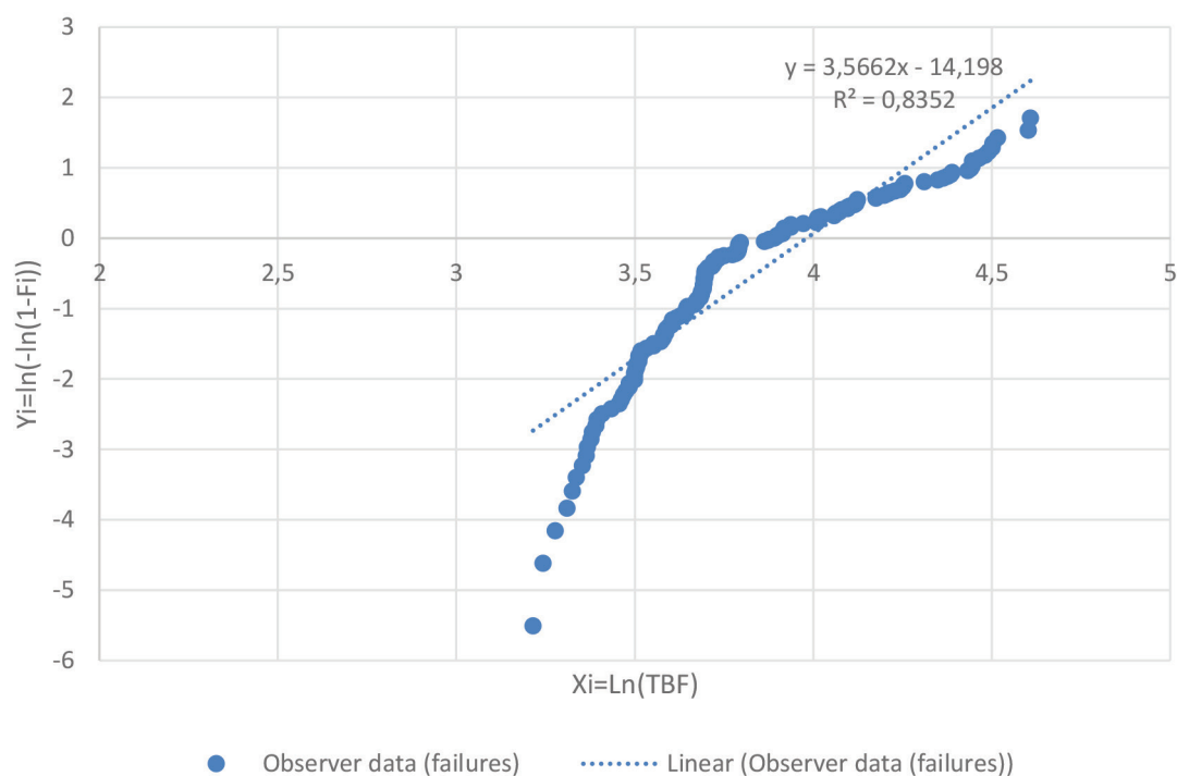
Figure 3. Weibull probability plot for Wood Chipper 1.
