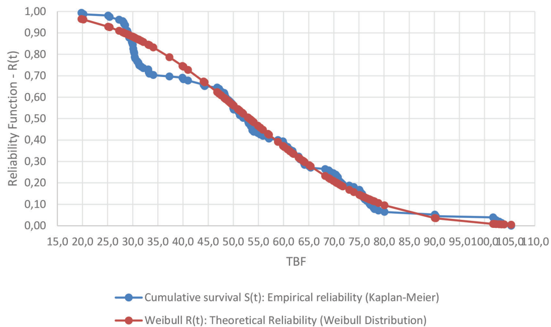
Figure 11. Comparison between the Kaplan–Meier survival curve and the Weibull model for the Wood Chipper 2.
