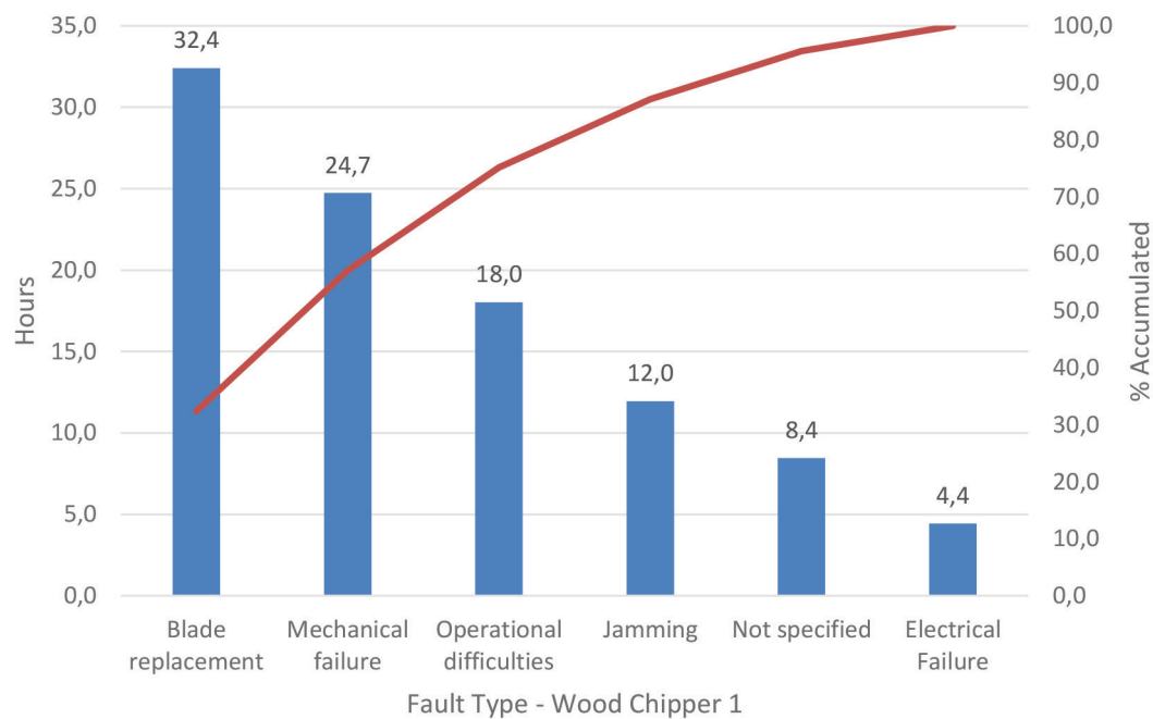
Figure 5. Analysis of various types of Wood Chipper 1 failures using the Pareto Diagram.
