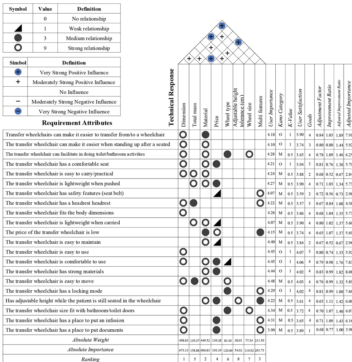
Figure 4. House of Quality Matrix
